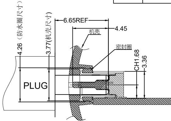
RECOMMENDED ASSEMBLY DRAWING
