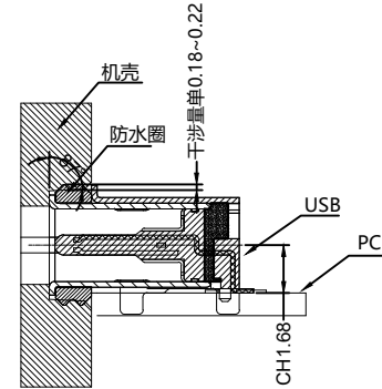
RECOMMENDED ASSEMBLY DRAWING
